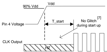
Figure 4. Startup Timing (OE/ST Mode)
