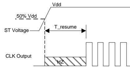
Figure 5. Standby Resume Timing (ST Mode Only)
